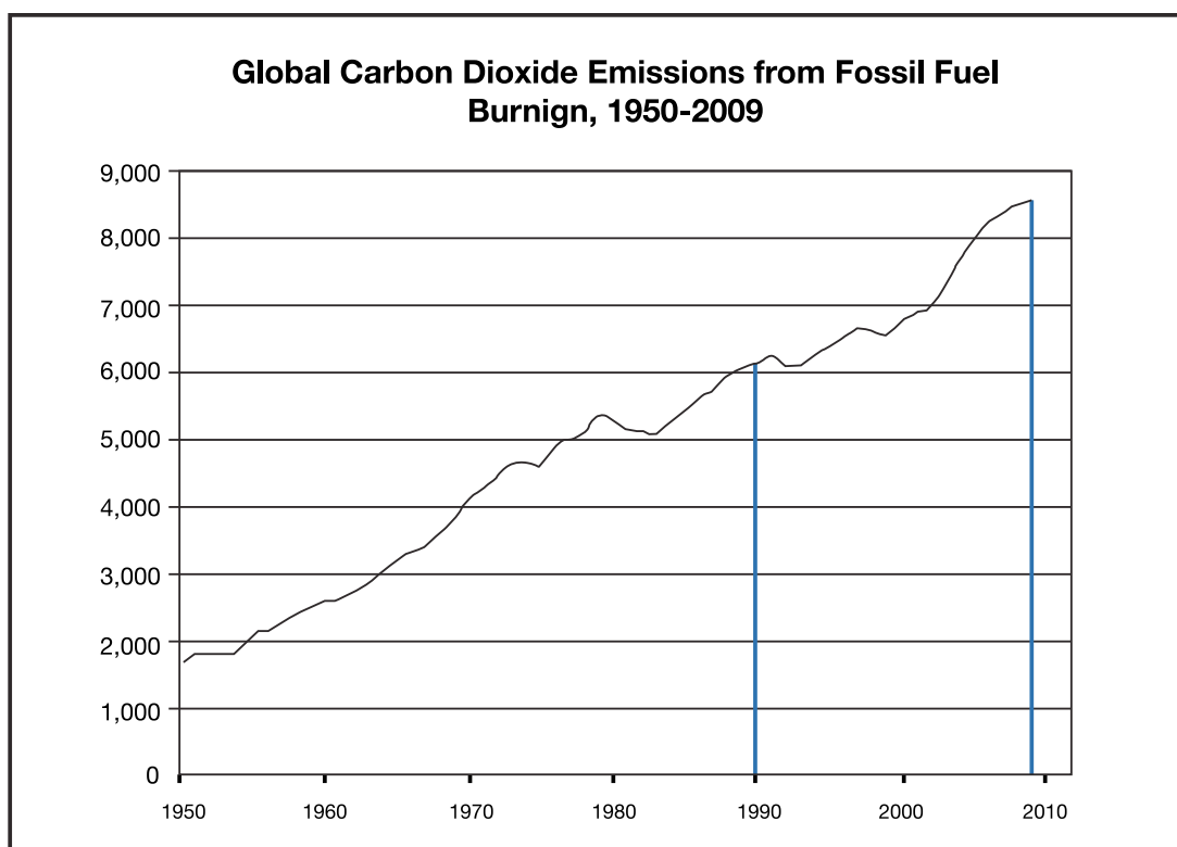
Graph 6 : Annual CO 2 emissions: 1950-2009
